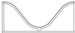
SINUS wave valley MGR 03.0002 P x L x K 180 x 90 x 80 cm
